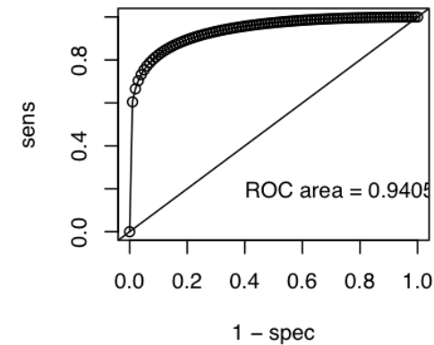
ROC Curve
