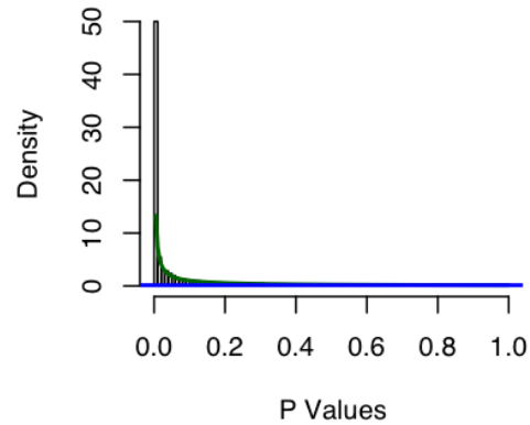
Beta-Uniform Mixture
