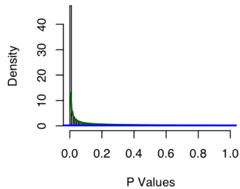
Beta-Uniform Mixture
