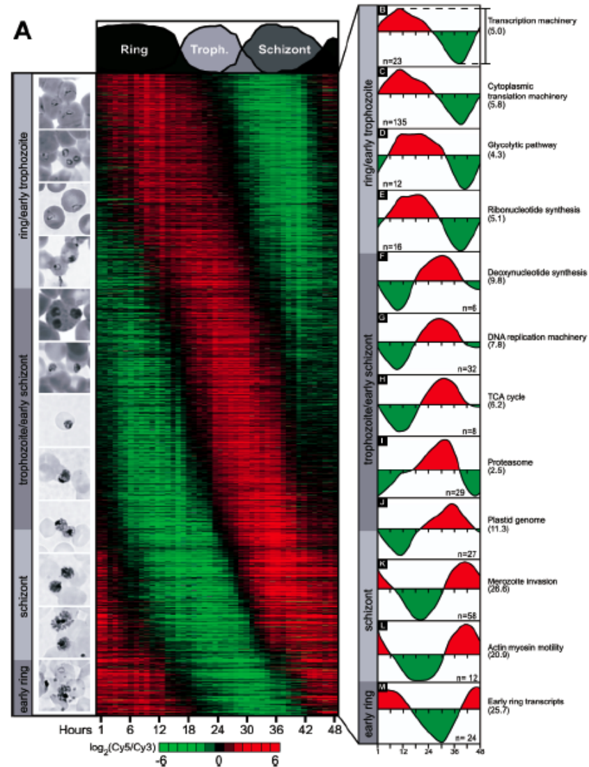
Figure 2. Overview of the P. falciparum IDC Transcriptome
