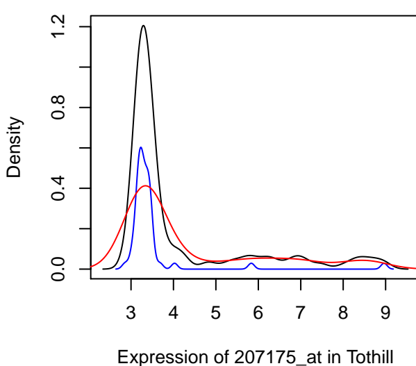
Density of 207175_at in Tothill
