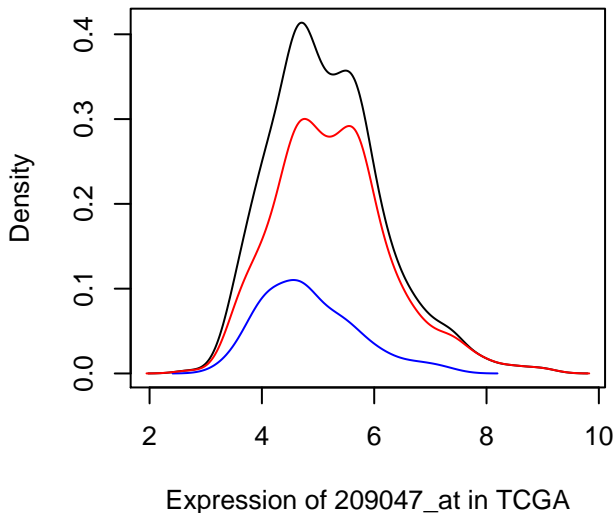
Density of 209047_at in TCGA
