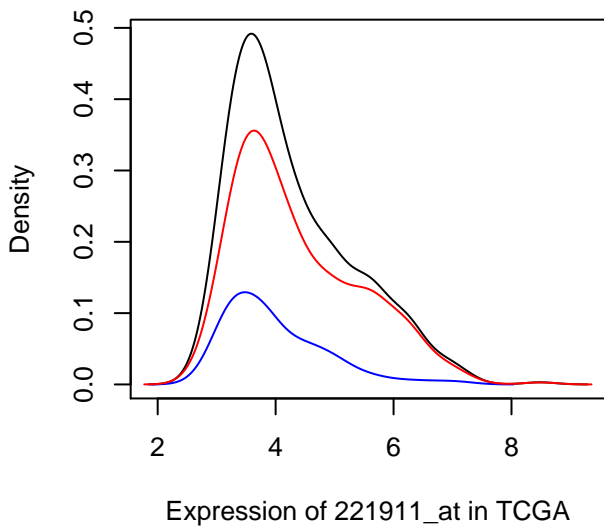
Density of 221911_at in TCGA
