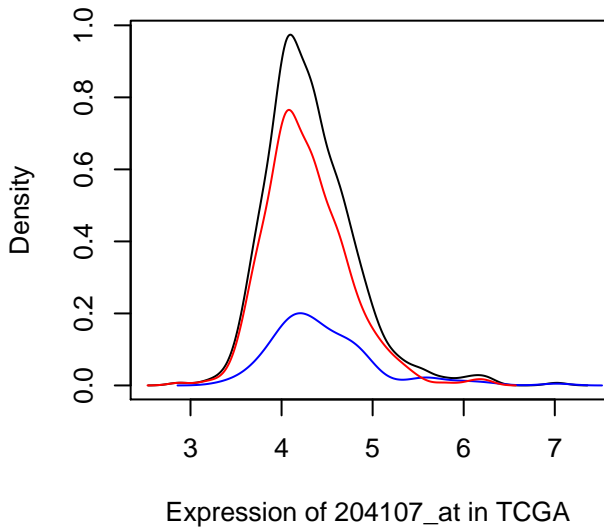
Density of 204107_at in TCGA
