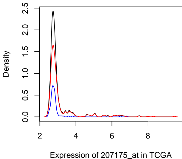
Density of 207175_at in TCGA
