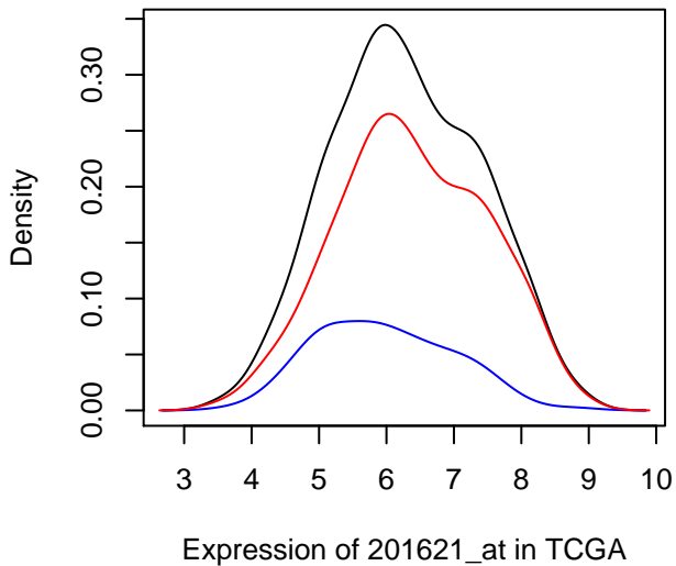
Density of 201621_at in TCGA
