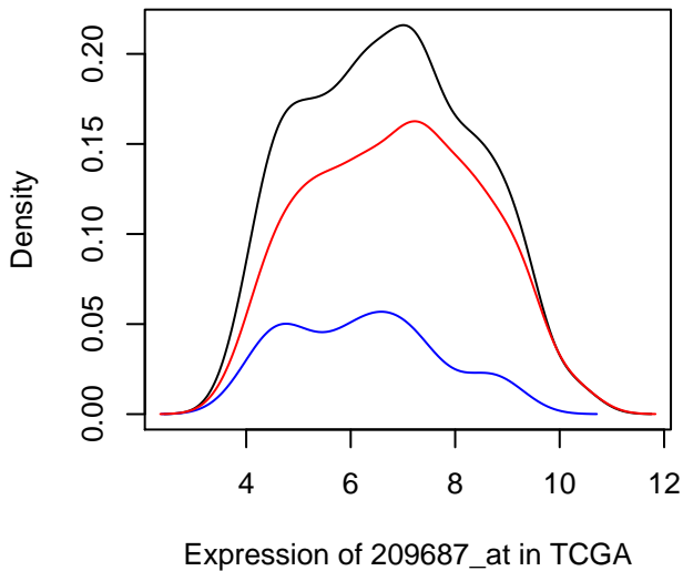
Density of 209687_at in TCGA
