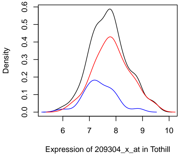
Density of 209304_x_at in Tothill
